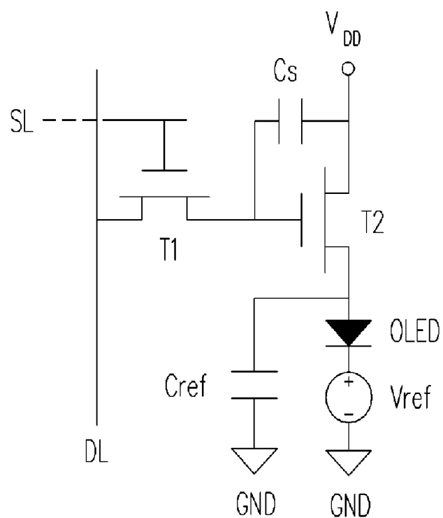
FIG. 5 (PRIOR ART)
